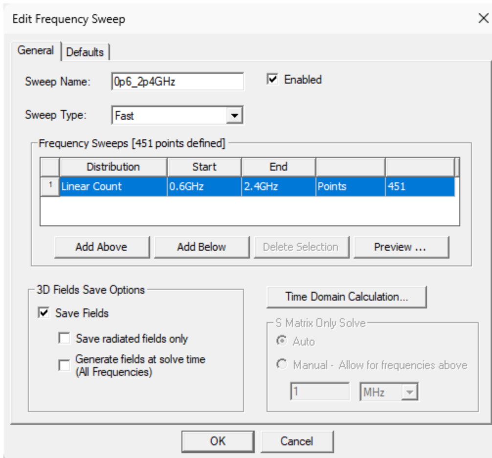
Figure 4-3: Edit Frequency Sweep Dialog Box
