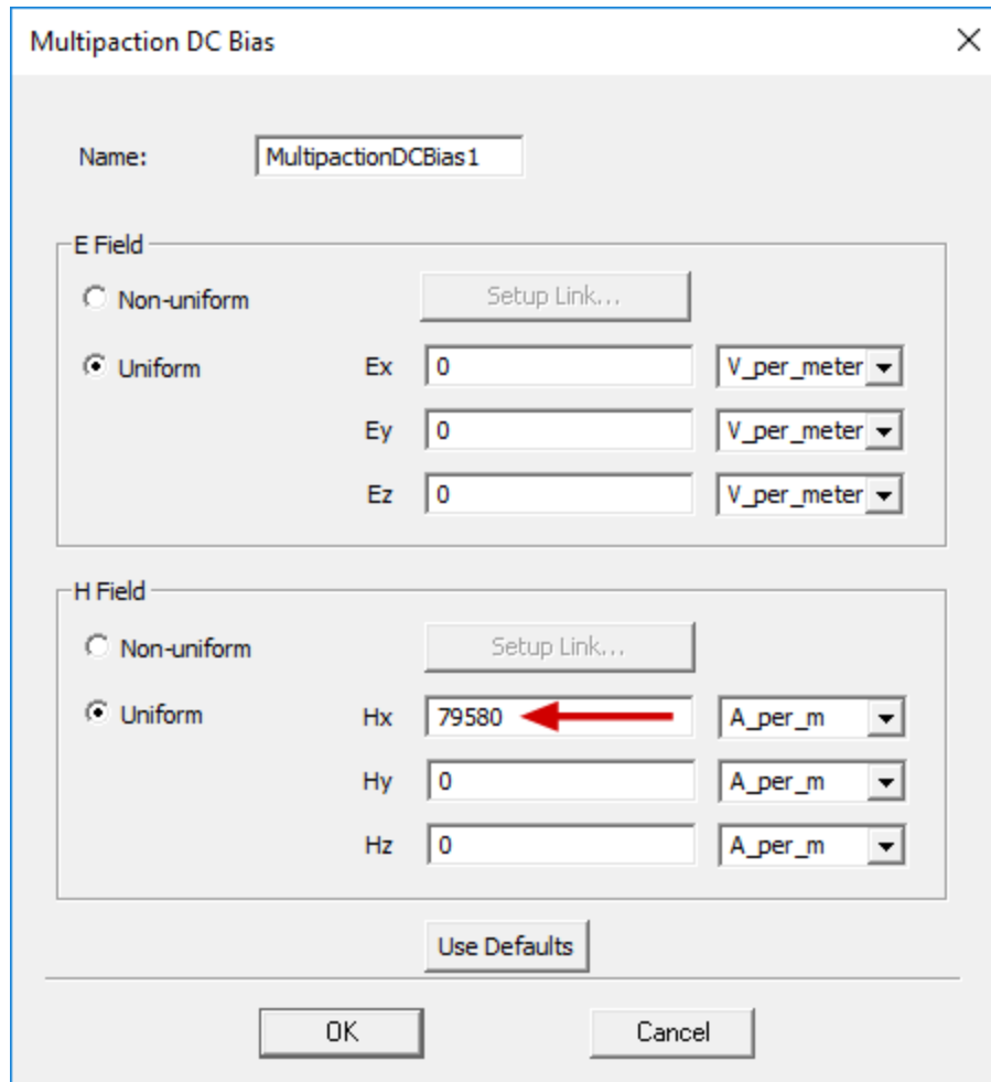
Figure 6-27: Multipaction DC Bias Dialog Box
