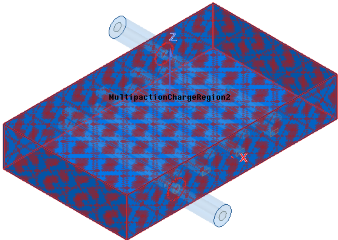
Figure 6-13: Multipaction Charge Region 2 Assigned
